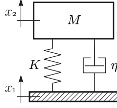
Figure 2: SDOF system mass-spring-dashpot with ground excitation.
