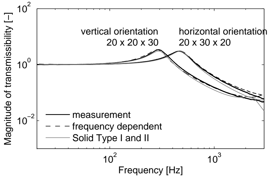
Figure 10: Comparison of transmissibilities calculated with frequency-dependent Young’s modulus and damping and constant Young’s modulus and damping obtained from Solid Type I and II model with measurement for specimen 2 with a horizontal (cross-section 20 mm x 30 mm) and vertical orientations (cross-section 20 mm x 20 mm).
