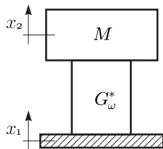
Figure 1: Single-degree-of-freedom (SDOF) system with ground excitation.
