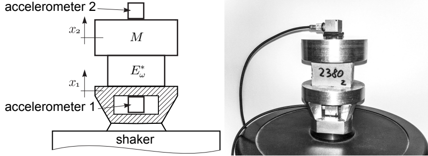
Figure 3: Experimental set-up.
