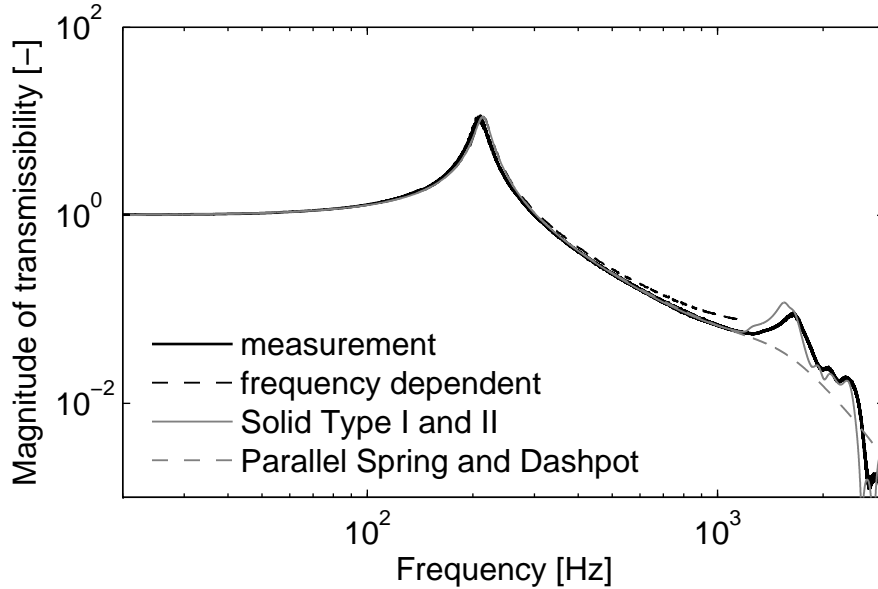
Figure 8: Comparison of transmissibilities calculated with frequency-dependent Young’s modulus and damping, constant Young’s modulus and damping obtained from Solid Type I and II model and from Parallel Spring and Dashpot model with measurement for specimen 1 with a horizontal orientation (cross-section 20 mm x 30 mm).
