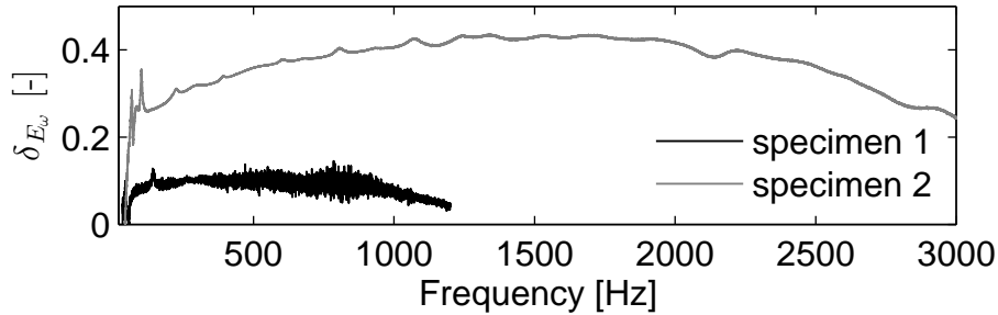
Figure 5: Damping factor as a function of frequency for specimen 1 (rubber of hardness 40 ShA) and specimen 2 (rubber of hardness 63 ShA).
