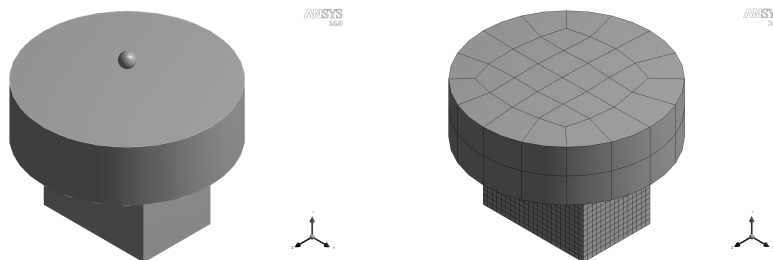
Figure 7: Finite element model in ANSYS Workbench v.14, model (left) and mesh (right).
