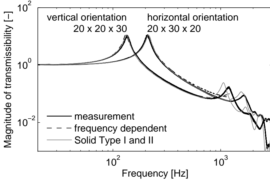
Figure 9: Comparison of transmissibilities calculated with frequency-dependent Young’s modulus and damping and constant Young’s modulus and damping obtained from Solid Type I and II model with measurement for specimen 1 with a horizontal (cross-section 20 mm x 30 mm) and vertical orientations (cross-section 20 mm x 20 mm).
