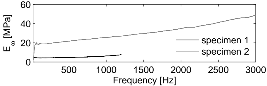
Figure 4: Young's modulus as a function of frequency for specimen 1 (rubber of hardness 40 ShA) and specimen 2 (rubber of hardness 63 ShA).
